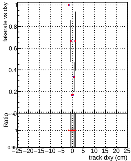
Fake rate vs d —●— DQM V0001_R0000000001 Global CMSSW_X_Y_Z alINODNN2 —●— DQM V0001_R0000000001 Global CMSSW_X_Y_Z all2
