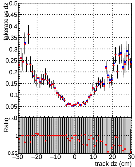
—●— DQM_V0001_R0000000001 Global CMSSW X Y Z alINODNN2 —●— DQM_V0001_R0000000001 Global CMSSW X Y Z all2
