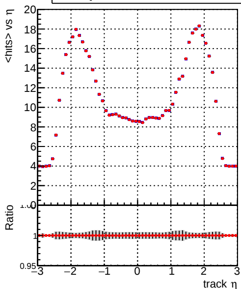
— DQM_V0001_R000000001_Global_CMSSW_X_Y_Z_allNODNN2 — DQM_V0001_R000000001_Global_CMSSW_X_Y_Z_all2
