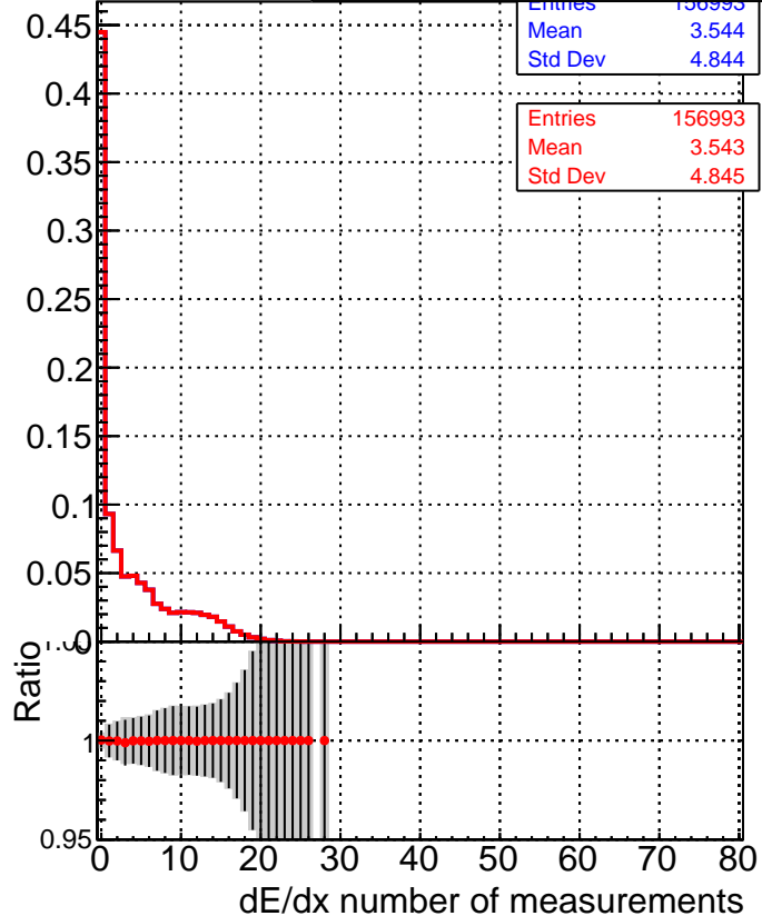
█ DQM_V0001_R000000001_Global_CMSSW_X_Y_Z_allNODNN2 —●— DQM_V0001_R000000001_Global_CMSSW_X_Y_Z_all2
