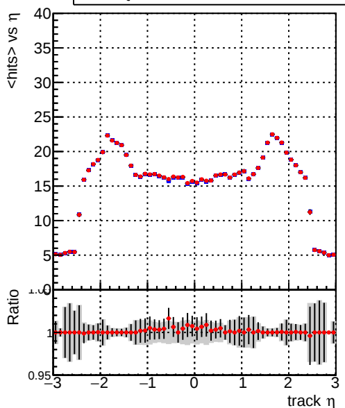
mean hits vs \eta — DQM_V0001_R000000001_Global_CMSSW_X_Y_Z_allNODNN2 — DQM_V0001_R000000001_Global_CMSSW_X_Y_Z_all2
