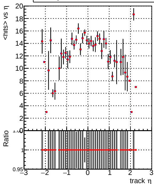
mean hits Legend: DQM_V0001_R000000001_Global_CMSSW_X_Y_Z_allNODNN2 (blue line), DQM_V0001_R000000001_Global_CMSSW_X_Y_Z_all2 (red line)
