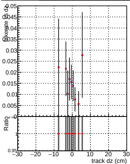
Global CMSSW X Y Z allNODNN2 Fake rate vs d —●— —●— —●— Duplicates Rate vs d —●— —●— —●— Pileup rate vs d —●— —●— —●—
