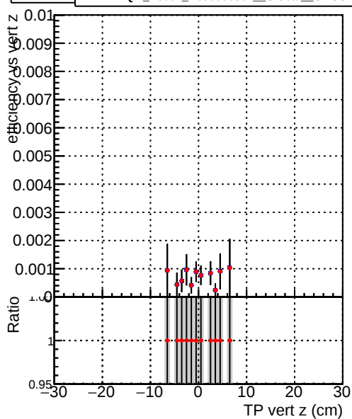
Efficiency — DQM_V0001_R000000001_Global_CMSSW_X_Y_Z_all2
