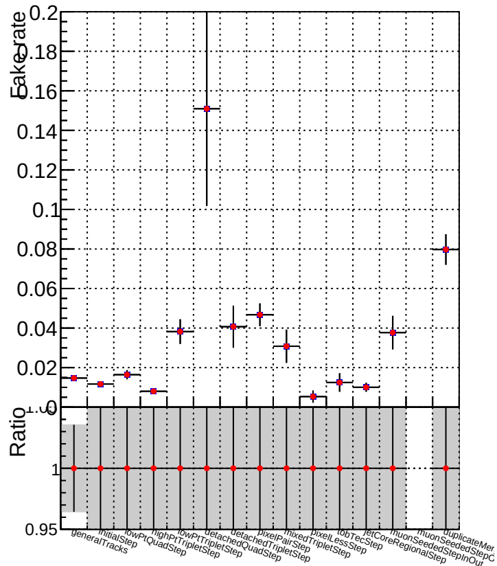
DQM_V0001_R000000001_Global_CMSSW_X_Y_Z_allNODNN2 DQM_V0001_R000000001_Global_CMSSW_X_Y_Z_all2
