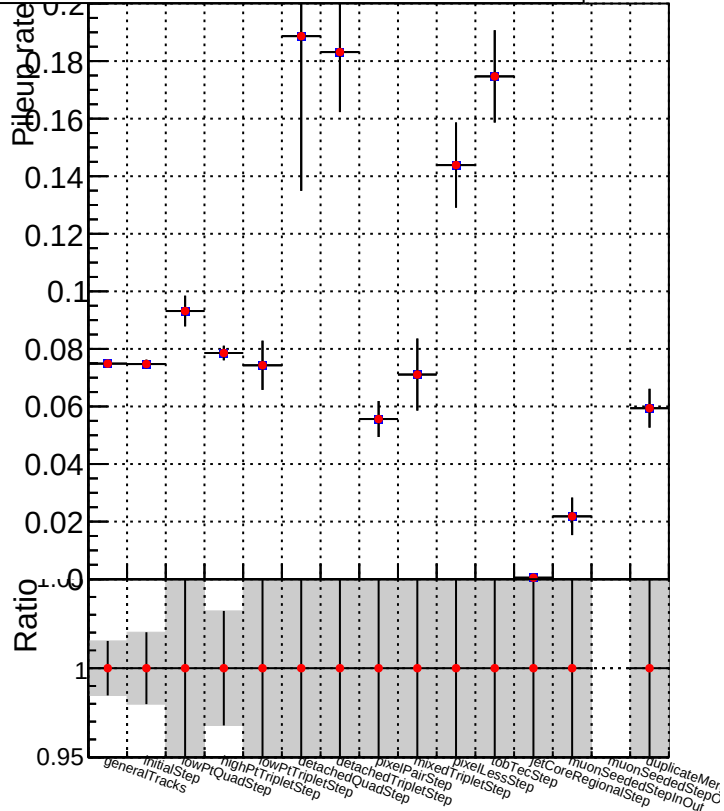
DQM_V0001_R000000001_Global_CMSSW_X_Y_Z_allNODNN2 DQM_V0001_R000000001_Global_CMSSW_X_Y_Z_all2
