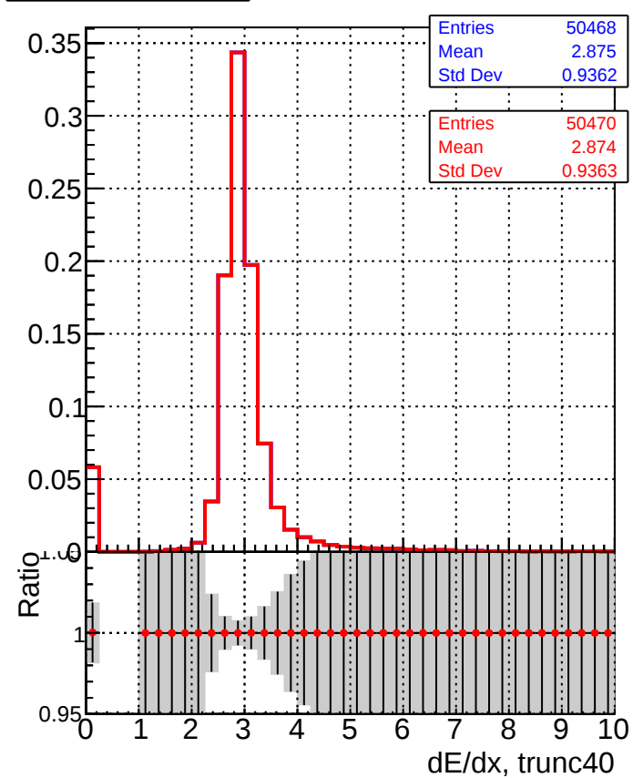
DQM_V0001_R000000001_Global_CMSSW_X_Y_Z_allNODNN2 DQM_V0001_R000000001_Global_CMSSW_X_Y_Z_all2
