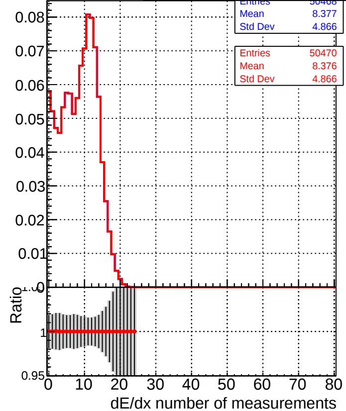
DQM_V0001_R000000001_Global_CMSSW_X_Y_Z_allNODNN2 DQM_V0001_R000000001_Global_CMSSW_X_Y_Z_all2
