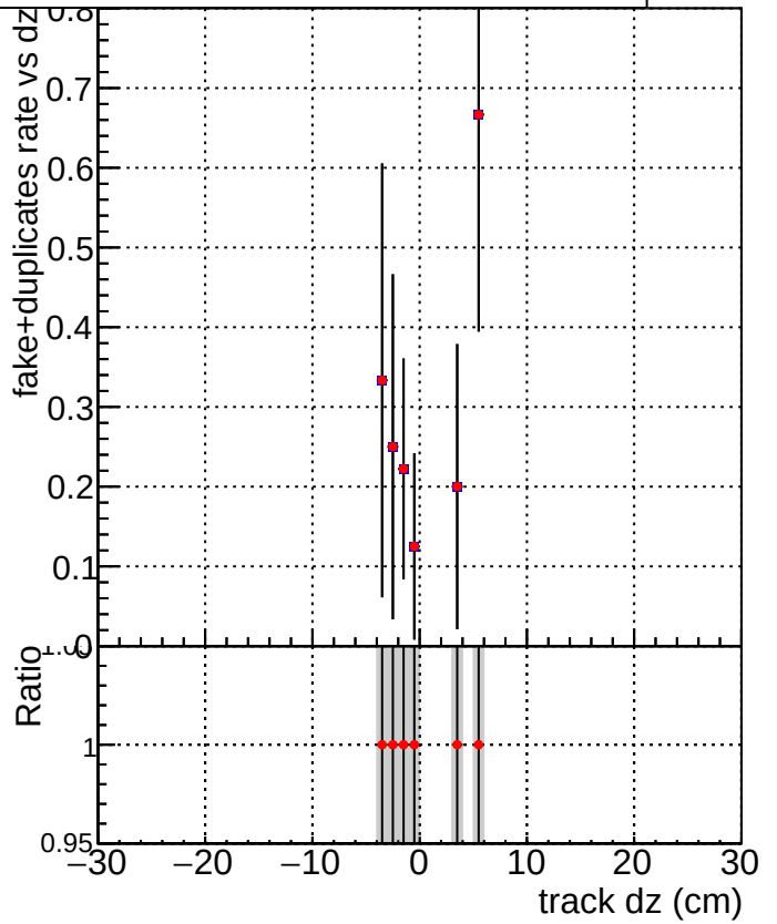
DQM_V0001_R000000001_Global_CMSSW_X_Y_Z_allINODNN2 DQM_V0001_R000000001_Global_CMSSW_X_Y_Z_all2
