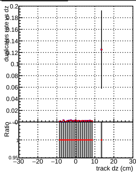
—●— DQM_V0001_R0000000001 Global CMSSW_X_Y_Z allNODNN2 —●— DQM_V0001_R0000000001 Global CMSSW_X_Y_Z all2
