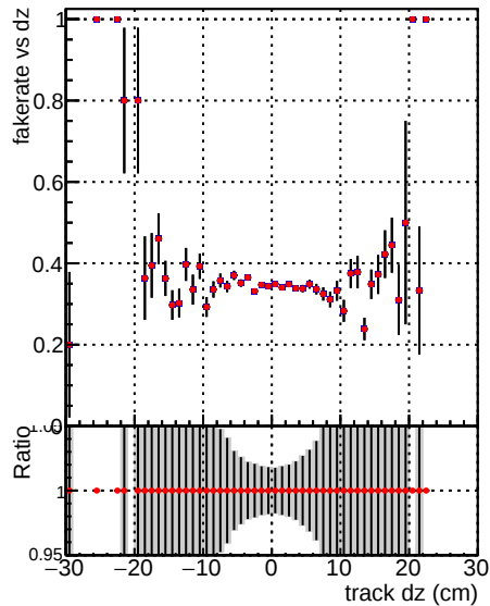
Fake rate vs dz —●— DQM_V0001_R0000000001 Global CMSSW_X_Y_Z alINODNN2 —●— DQM_V0001_R0000000001 Global CMSSW_X_Y_Z all2
