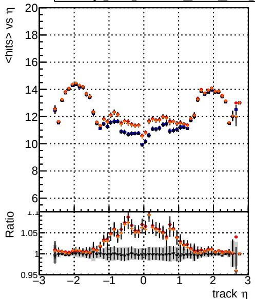
mean hits vs \eta Legend: DQM_V0001_R000000001_Global_mkFit_1kstable DQM_V0001_R000000001_Global_mkFit_CAND1kstable DQM_V0001_R000000001_Global_mkFit_1kswitch DQM_V0001_R000000001_Global_mkFit_CAND1kswitch
