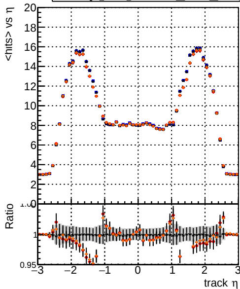
mean hits vs \eta DQM_V0001_R000000001_Global_mkFit_1kstable DQM_V0001_R000000001_Global_mkFit_CAND1kstable DQM_V0001_R000000001_Global_mkFit_1kswitch DQM_V0001_R000000001_Global_mkFit_CAND1kswitch
