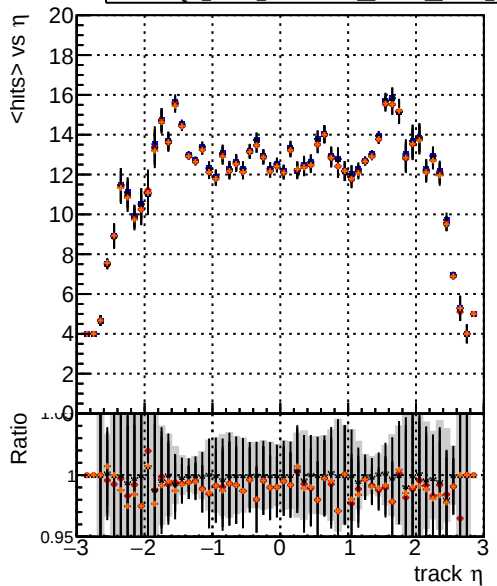
mean hits vs \eta DQM_V0001_R000000001_Global_mkFit_1kstable DQM_V0001_R000000001_Global_mkFit_CAND1kstable DQM_V0001_R000000001_Global_mkFit_1kswitch DQM_V0001_R000000001_Global_mkFit_CAND1kswitch
