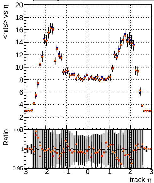
mean hit DQM_V0001_R0000000001 Global mkFit_1kstable DQM_V0001_R0000000001 Global mkFit_CAND1kstable DQM_V0001_R0000000001 Global mkFit_1kswitch DQM_V0001_R0000000001 Global mkFit_CAND1kswitch
