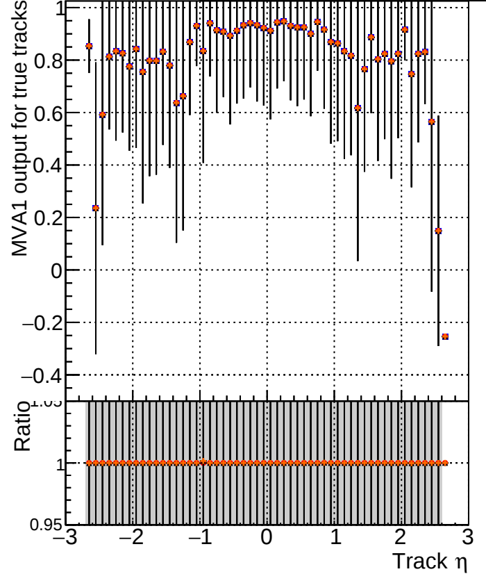
MVA1 of associated tracks (recoToSim) vs. track \eta █ DQM_V0001_R0000000001 Global mkFit_1kstable ● DQM_V0001_R0000000001 Global mkFit_CAND1kstable ▲ DQM_V0001_R0000000001 Global mkFit_1kswitch ◆ DQM_V0001_R0000000001 Global mkFit_CAND1kswitch
