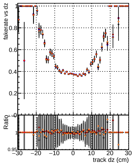
Fake rate vs d DGM V0001 1kstable Global mkFit 1kstable CANDID 1kstable
