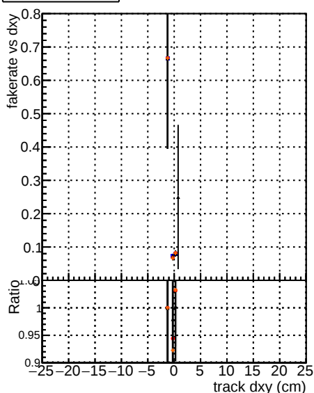
Fake rate vs d DGM V0001 DGM V0001 DGM V0001 Global mkFit 1kstable DGM V0001 DGM V0001 DGM V0001 Global mkFit CANDID 1kstable DGM V0001 DGM V0001 DGM V0001 Global mkFit CANDID switch
