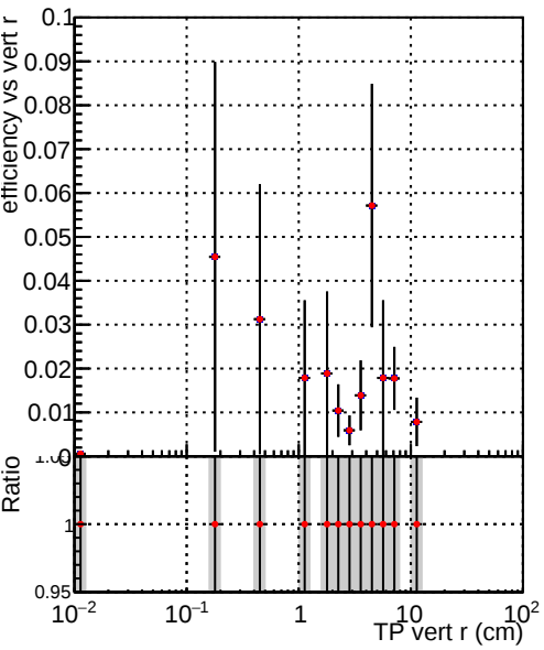
Efficiency vs vertpos Legend: DQM_V0001_R0000000001_Global_mkFit_CAND100stable DQM_V0001_R0000000001_Global_mkFit_CANDFINAL100stable
