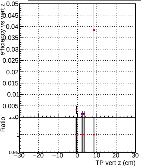
Efficiency vs. TP vert z (cm) Legend: DQM_V0001_R000000001_Global_mkFit_CAND100stable DQM_V0001_R000000001_Global_mkFit_CANDFINAL100stable
