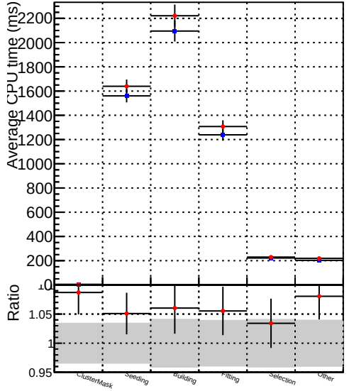
Average CPU time / event Legend: ■ DQM_V0001_R000000001_Global_mkFit_CAND100stable ■ DQM_V0001_R000000001_Global_mkFit_CANDFINAL100stable
