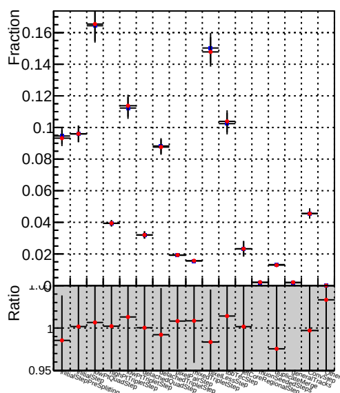
Average CPU time / event Legend: ■ DQM_V0001_R000000001_Global_mkFit_CAND100stable ■ DQM_V0001_R000000001_Global_mkFit_CANDFINAL100stable
