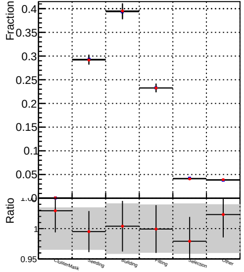
Average CPU time / event Legend: ■ DQM_V0001_R000000001_Global_mkFit_CAND100stable ■ DQM_V0001_R000000001_Global_mkFit_CANDFINAL100stable
