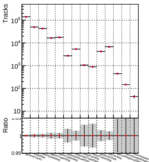
DQM_V0001_R000000001_Global_mkFit_CAND100stable
