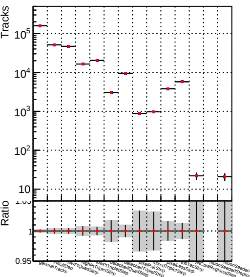
DQM_V0001_R000000001__Global__mkFit_CAND100stable
