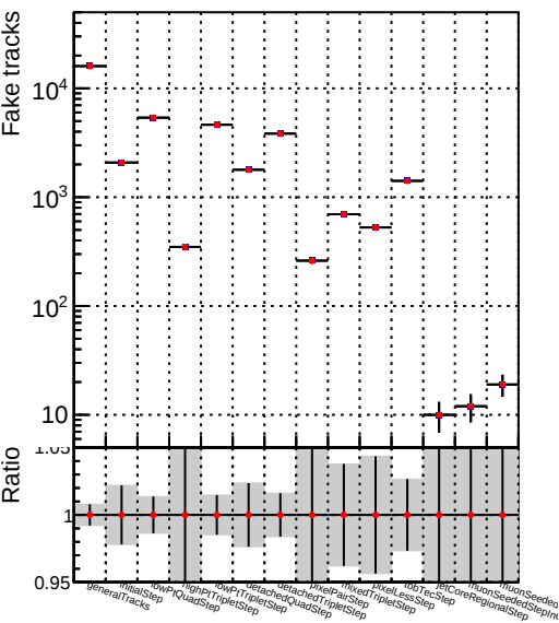
Number —● DQM_V0001_R000000001_Global_mkFit_CANDFINAL100stable
