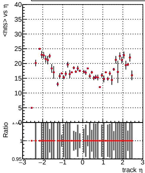
— DQM_V0001_R000000001_Global_mkFit_CAND100stable — DQM_V0001_R000000001_Global_mkFit_CANDFINAL100stable
