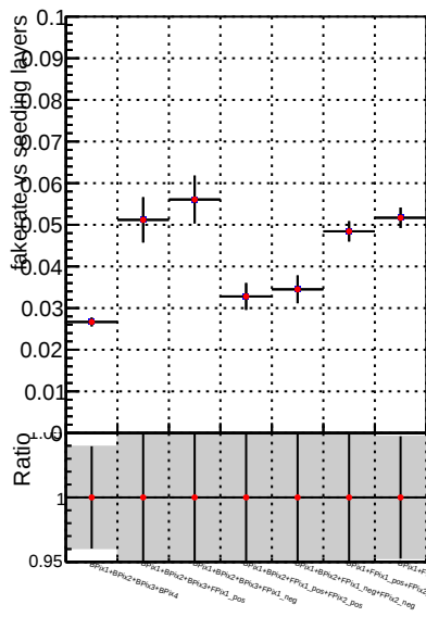
Fake rate vs. —●— DQM_V0001_R000000001_Global_mkFit_CAND100stable —●— DQM_V0001_R000000001_Global_mkFit_CANDFINAL100stable
