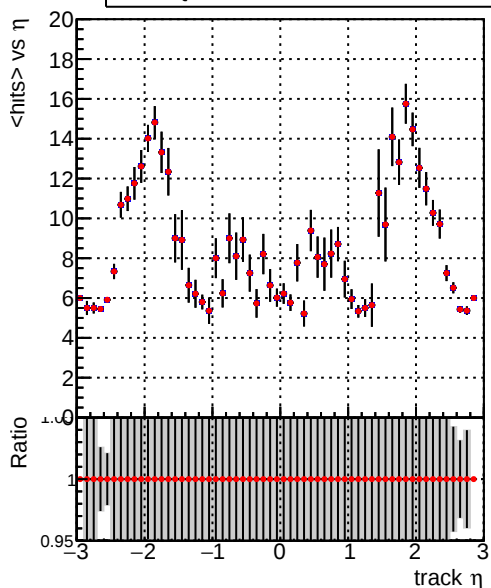
— DQM_V0001_R000000001_Global_mkFit_CAND100stable — DQM_V0001_R000000001_Global_mkFit_CANDFINAL100stable
