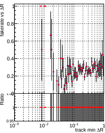
Legend: \blacksquare DQM_V0001_R000000001_Global_mkFit_CAND100stable \bullet DQM_V0001_R000000001_Global_mkFit_CANDFINAL100stable
