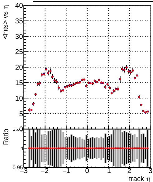
mean hit — DQM_V0001_R000000001_Global_mkFit_CAND100stable — DQM_V0001_R000000001_Global_mkFit_CANDFINAL100stable
