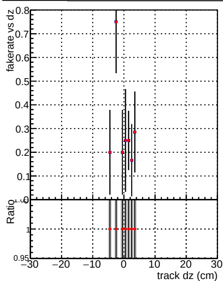
—•— DQM_V0001_R0000000001_Global_mkFit_CAND100stable —•— DQM_V0001_R0000000001_Global_mkFit_CANDFINAL100stable
