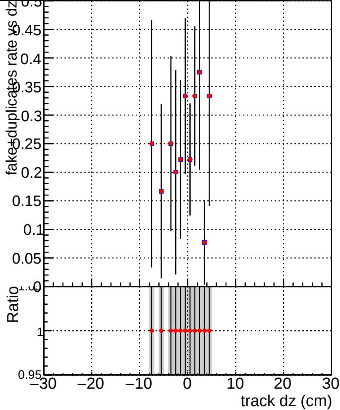
DQM_V0001_R0000000001_Global_mkFit_CAND100stable DQM_V0001_R0000000001_Global_mkFit_CANDFINAL100stable
