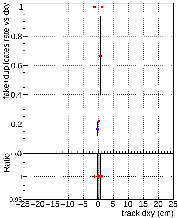
DQM_V0001_R0000000001_Global_mkFit_CAND100stable DQM_V0001_R0000000001_Global_mkFit_CANDFINAL100stable
