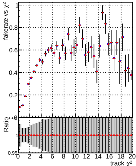
Fake rate vs. —•— DQM_V0001_R000000001_Global_mkFit_CAND100stable —•— DQM_V0001_R000000001_Global_mkFit_CANDFINAL100stable
