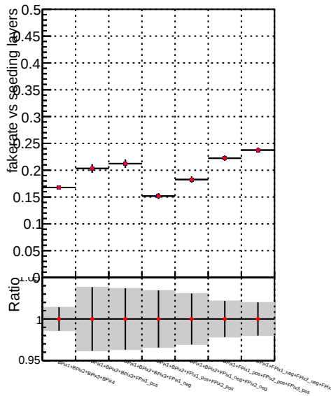
Fake rate vs. —•— DQM_V0001_R000000001_Global_mkFit_CAND100stable —•— DQM_V0001_R000000001_Global_mkFit_CANDFINAL100stable
