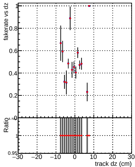
Fake rate vs dz —●— DQM_V0001_R0000000001_Global_mkFit_CAND100stable —●— DQM_V0001_R0000000001_Global_mkFit_CANDFINAL100stable
