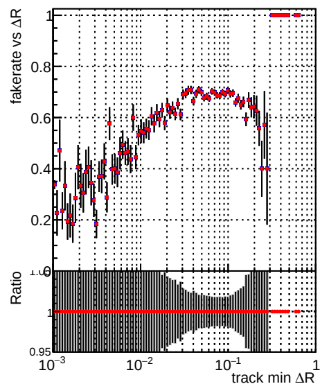
—●— DQM_V0001_R000000001_Global_mkFit_CAND100stable —●— DQM_V0001_R000000001_Global_mkFit_CANDFINAL100stable
