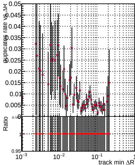
—●— DQM_V0001_R000000001_Global_mkFit_CAND100stable —●— DQM_V0001_R000000001_Global_mkFit_CANDFINAL100stable
