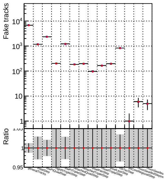
Number —● DQM_V0001_R000000001_Global_mkFit_CANDFINAL100stable
