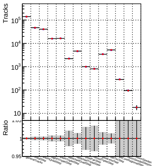
DQM_V0001_R000000001__Global__mkFit_CAND100stable
