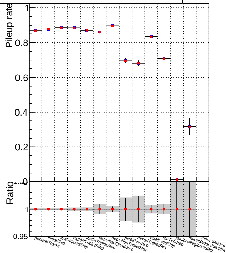
DQM_V0001_R000000001_Global_mkFit_CAND100stable
