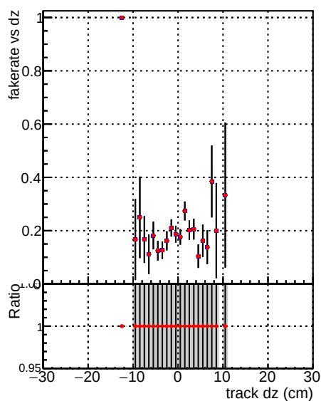
Fake rate vs dz —●— DQM_V0001_R0000000001_Global_mkFit_CAND100stable —●— DQM_V0001_R0000000001_Global_mkFit_CANDFINAL100stable
