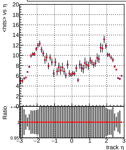
mean hits vs \eta Legend: DQM_V0001_R000000001_Global_mkFit_CAND100stable (blue line), DQM_V0001_R000000001_Global_mkFit_CANDFINAL100stable (red line)
