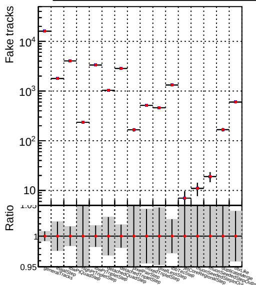
Number DOM V0001 R0000000001 Global mkFit CANDEFINAL 100stable2 1
