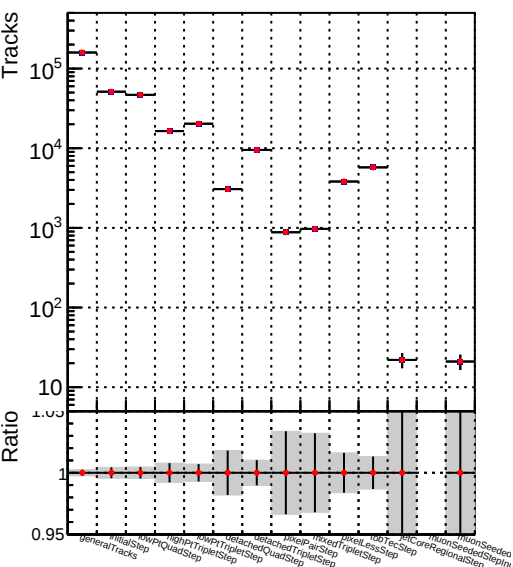
DQM_V0001_R000000001_Global_mkFit_CANDFINAL100stable
