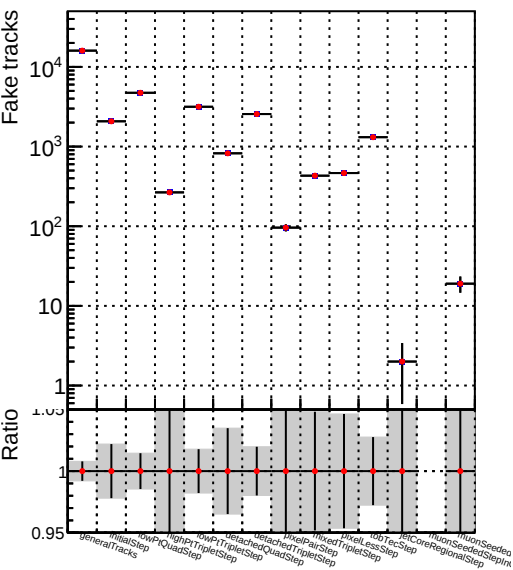
Number —●— DQM_V0001_R000000001_Global_mkFit_CANDFINAL100stable2
