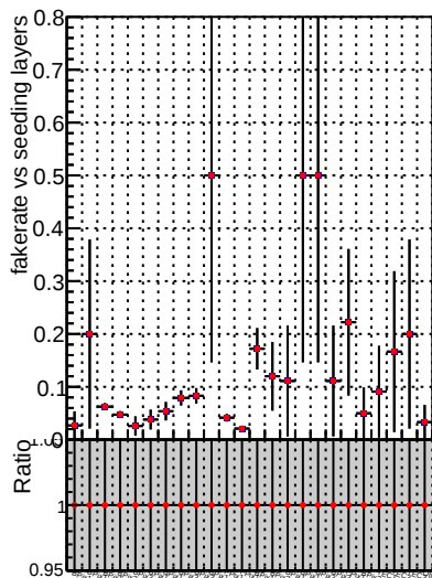
Fake rate vs. —●— DQM_V0001_R0000000001_Global_mkFit_CANDFINAL100stable —●— DQM_V0001_R0000000001_Global_mkFit_CANDFINAL100stable2
