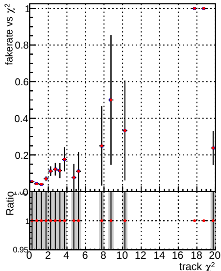
Fake rate vs. —●— DQM_V0001_R0000000001_Global_mkFit_CANDFINAL100stable —●— DQM_V0001_R0000000001_Global_mkFit_CANDFINAL100stable2
