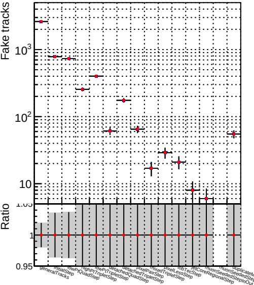
Number —●— DQM_V0001_R000000001_Global_mkFit_CANDFINAL100stable2
