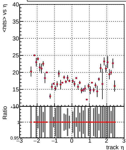
mean hit DQM_V0001_R000000001_Global_mkFit_CANDFINAL100stable DQM_V0001_R000000001_Global_mkFit_CANDFINAL100stable2
