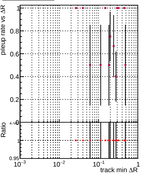
Legend: DQM_V0001_R000000001_Global_mkFit_CANDFINAL100stable DQM_V0001_R000000001_Global_mkFit_CANDFINAL100stable2
