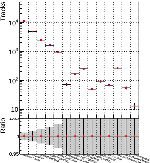
■ DQM_V0001_R000000001__Global__mkFit_CANDFINAL100stable
