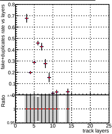
fake+duplicates rate vs layers
