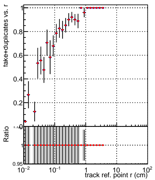
■ DQM_V0001_R000000001_Global_mkFit_CANDFINAL100stable ● DQM_V0001_R000000001_Global_mkFit_CANDFINAL100stable2
