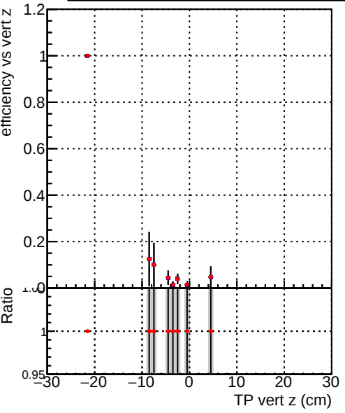
Efficiency vs vert z Legend: DQM_V0001_R0000000001_Global_mkFit_CANDFINAL100stable DQM_V0001_R0000000001_Global_mkFit_CANDFINAL100stable2
